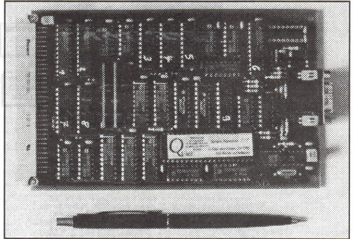
Above: The QVME Card: High quality construction. Below: The QVME Card fits nicely into the Atari STe.
